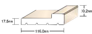
2×4・在来用折戸L型枠 EG3436 ℓ=3'-965 mm ¥3,300 7'-2135 mm ¥6,600
