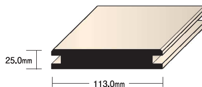
無目枠 RC104-21 ℓ = 2095 ㎜ ¥7,800
